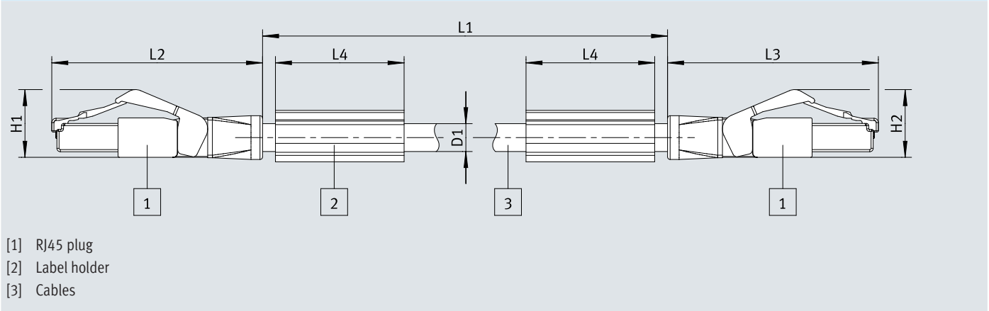
Dimensions – Plug RJ45 with plug RJ45, with snap-locking
