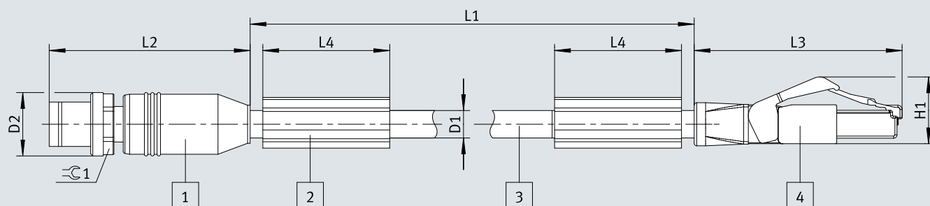
Dimensions – Plug M12 with plug RJ45, D-coded
