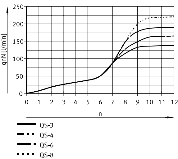
Standard nominal flow rate q_{nN} at 6 → 5 bar as a function of spindle revolutions n (GRLA/GRLZ-1/8 – push-in connector QS, metal)
