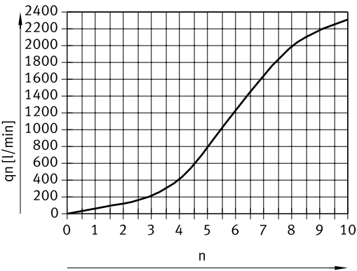
Standard flow rate q_n at 6 → 0 bar as a function of spindle revolutions n (GRLA/GRLZ-3/8 – female thread/barbed connector, metal)
