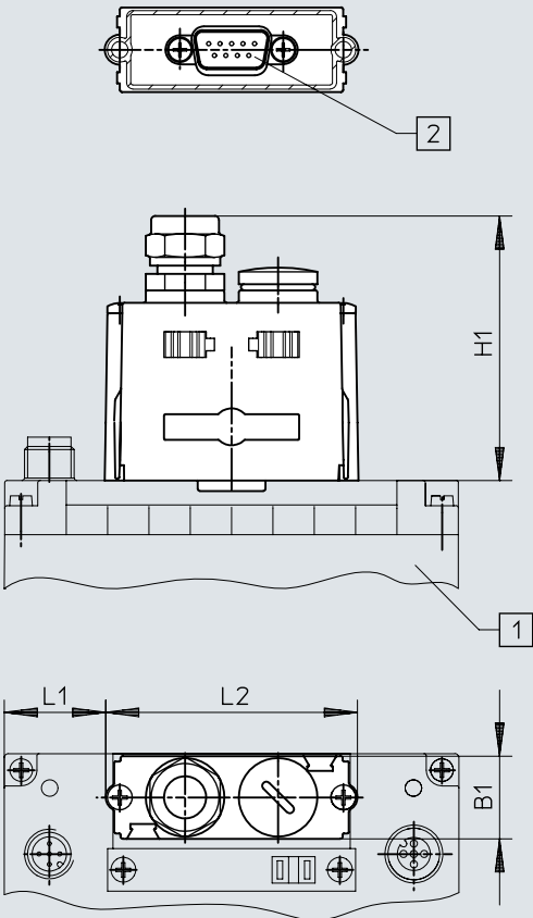
[1] Valve terminal with Fieldbus Direct CPV10/14/18 and bus node [2] Sub-D socket, 9-pin
