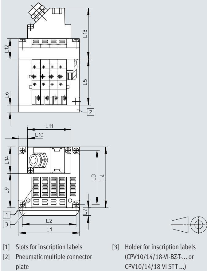
Valve terminal with multi-pin plug connection – CPV10/14/18
