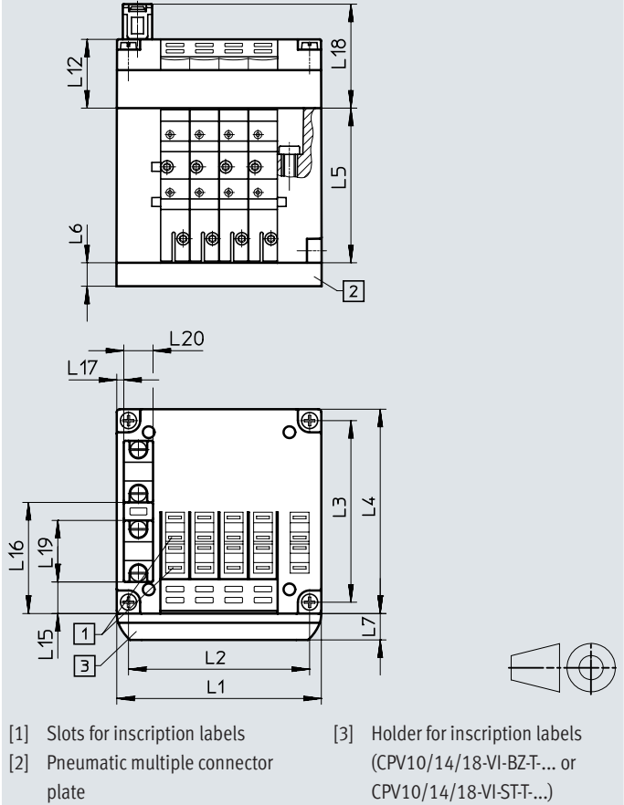
Valve terminal with AS-Interface connection – CPV10/14/18
