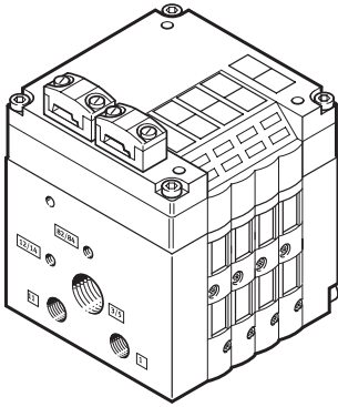
AS-Interface valve terminal with auxiliary power supply
