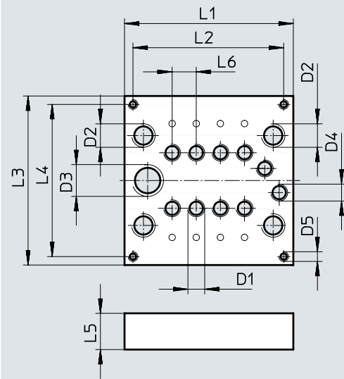
Pneumatic multiple connector plate – CPV10/14/18
