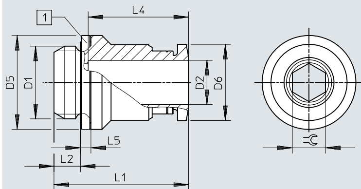
Dimensions – Push-in fitting QS-...-I, G-thread
