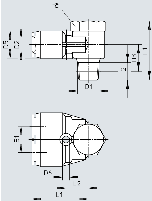
Dimensions – Push-in Y-fitting QSYLV, R thread
