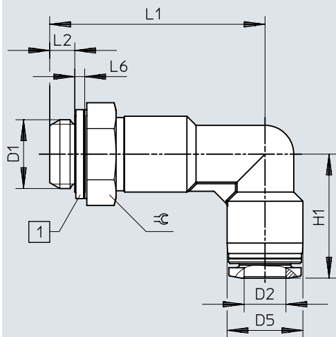
Dimensions – Push-in L-fitting, long, QSLL, G thread with sealing ring
