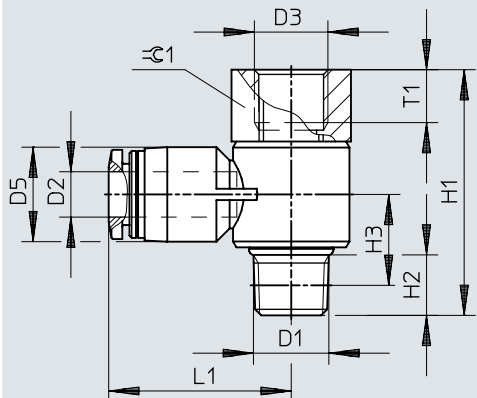
Dimensions – Push-in T-fitting QSTF, R thread
