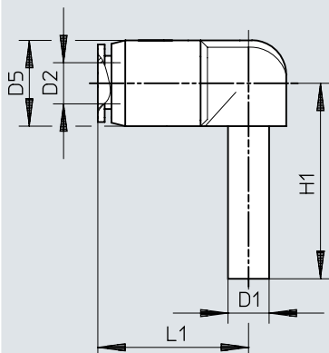
Dimensions – Push-in L-connector QSL-...HL with push-in sleeve
