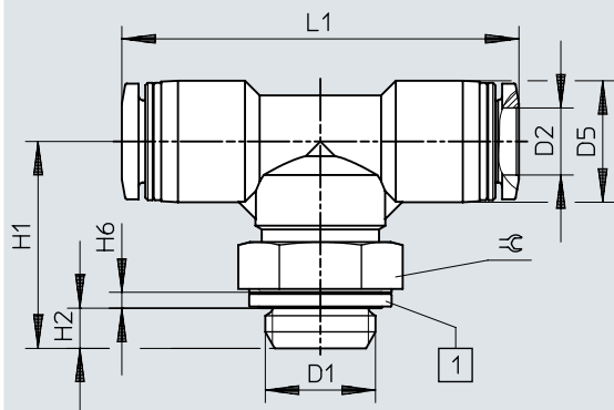
Dimensions – Push-in T-fitting QST, G-thread with sealing ring
