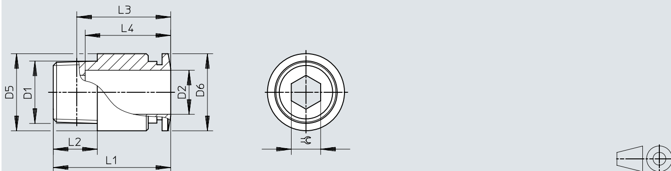
Dimensions – Push-in fitting QS-...-I, R thread
