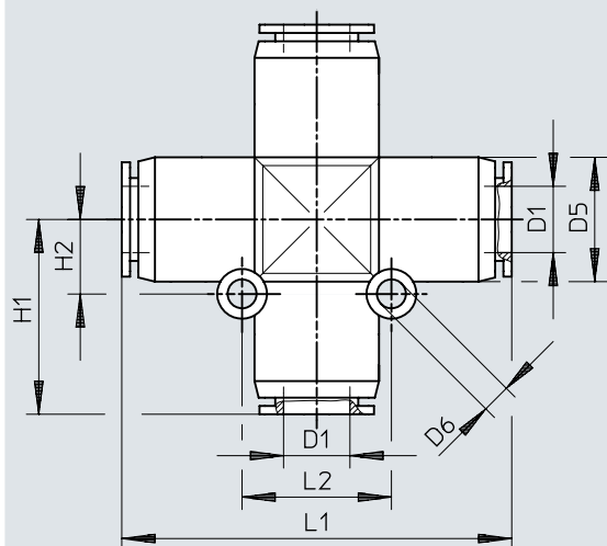
Dimensions – Push-in X-connector QSX
