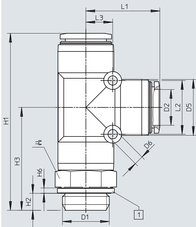
Dimensions – Push-in T-fitting QSTL-...-16, G thread with sealing ring
