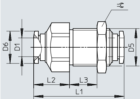
Dimensions – Push-in bulkhead connector QSS-...-F, with fixed collar
