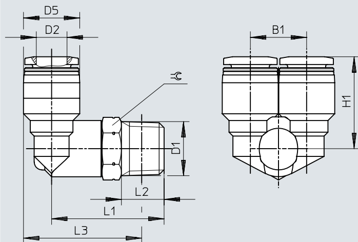
Dimensions – Push-in Y-fitting QSYL, R thread
