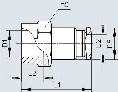
Dimensions – Push-in fitting QSF, G thread
