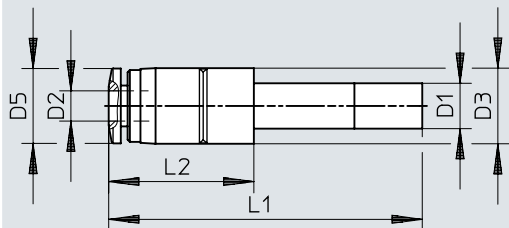
Dimensions – Push-in connector QS-...H
