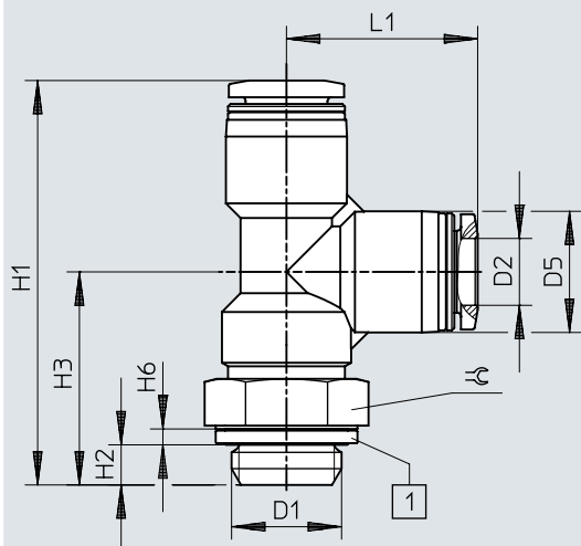
Dimensions – Push-in T-fitting QSTL, G thread with sealing ring
