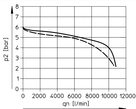
MS6-LR-1/2
