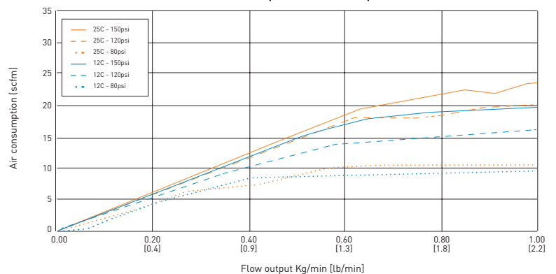
Air consumption vs flow output
