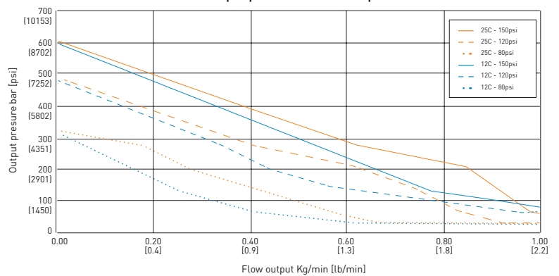
Output pressure vs flow output
