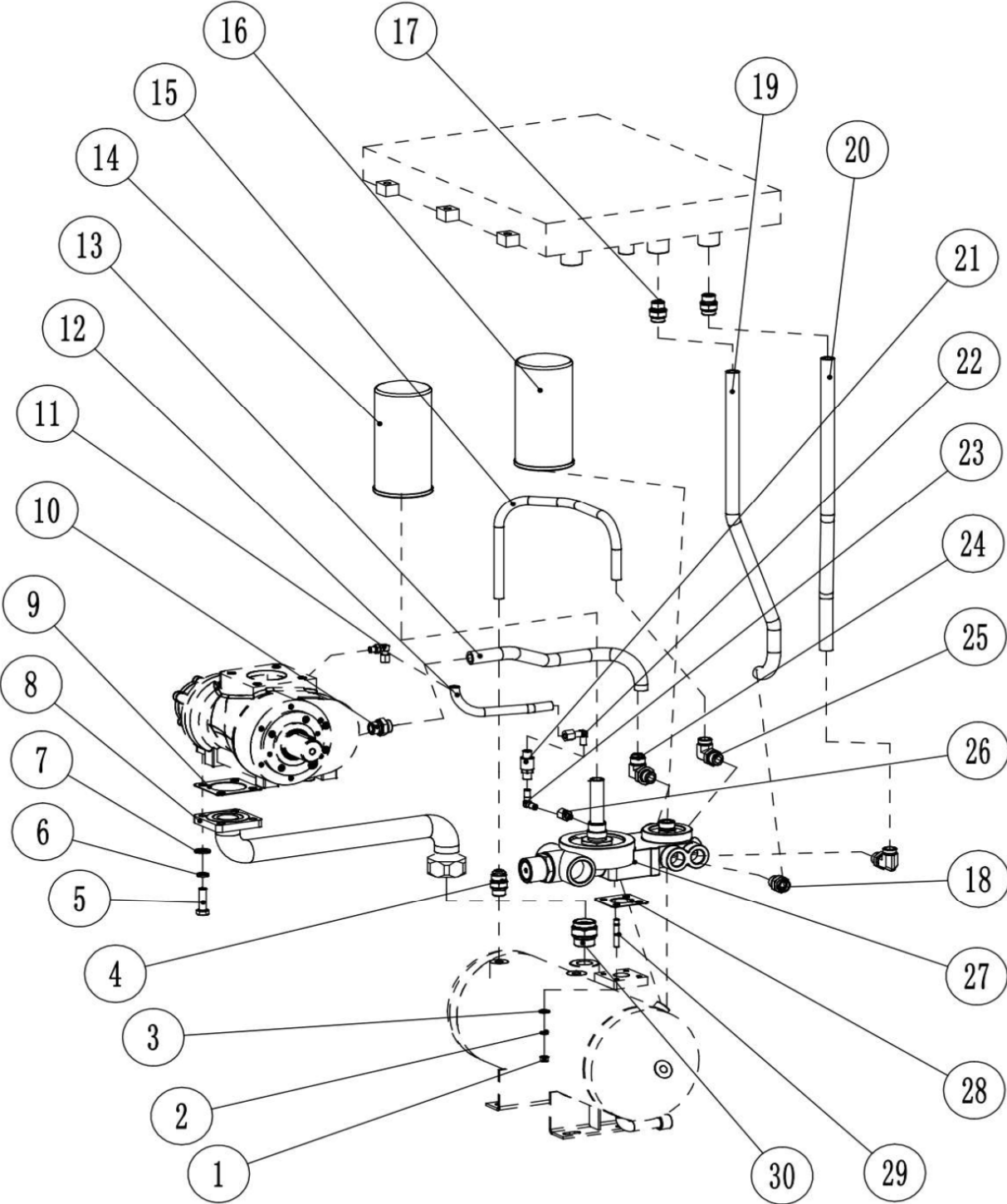
Model: GS(V)11/15 GS(V)11-15 Oil Circuit R00
