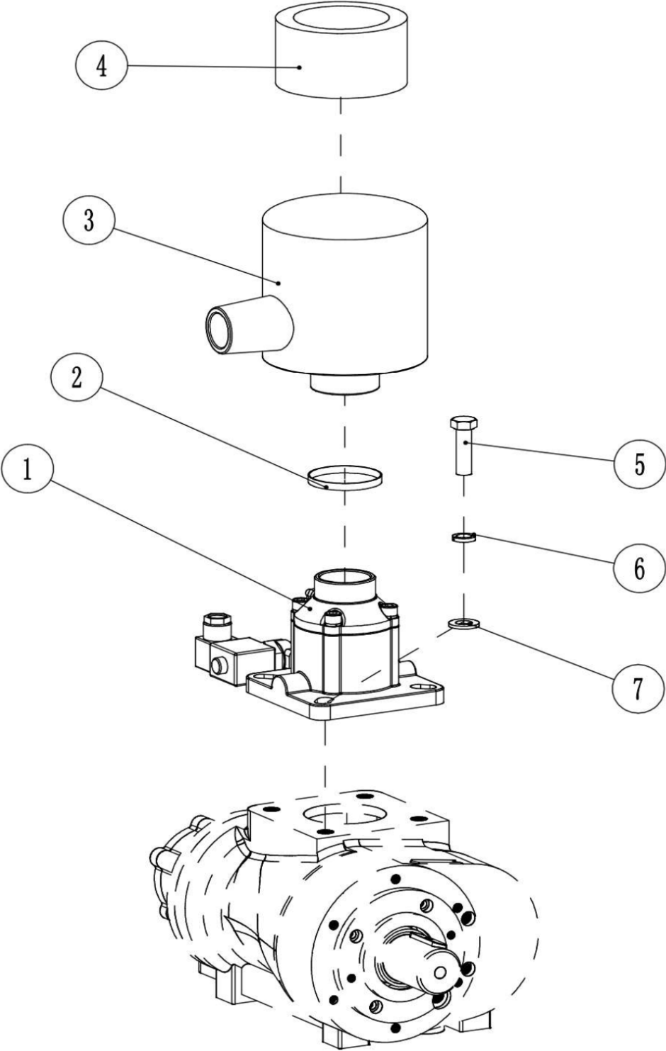
Model: GS(V)11/15 GS(V)11-15 Air Inlet R00
